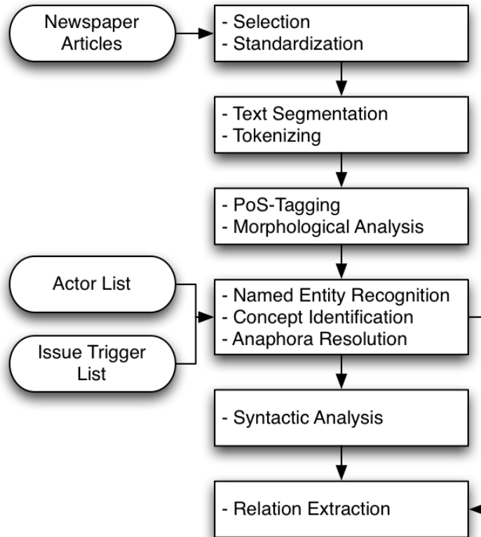
Figure 1: Software pipeline
